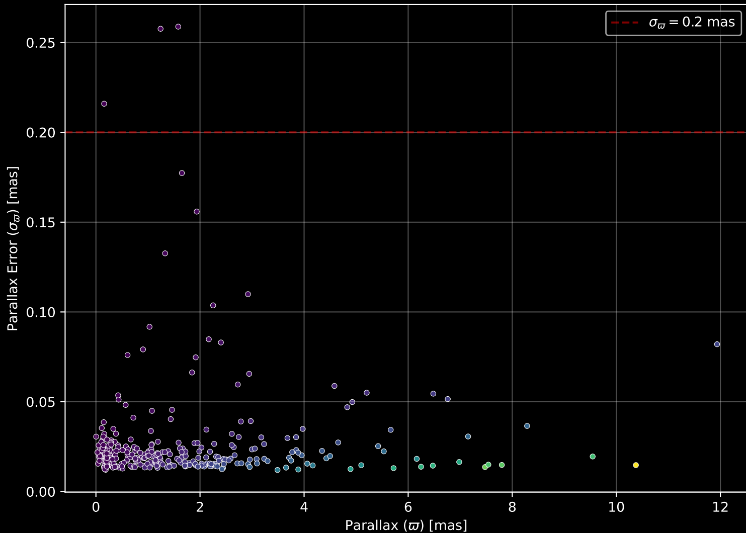
APOGEE DR17 Field: [M12-S] Parallax Quality (n= 321)
