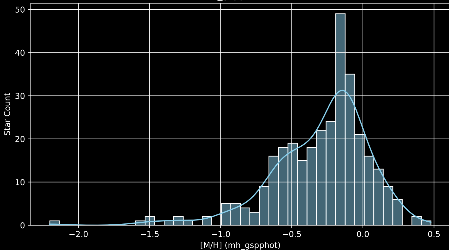
APOGEE DR17 Field: [M12-S [M/H] (mh_gspphot) (n= 320)
